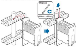
Figure 6-15 Installing the RRU on the pole
