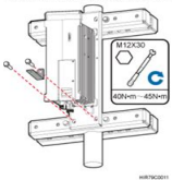
Figure 6-16 Installing the backplane the L plate on the lower mounting bracket
